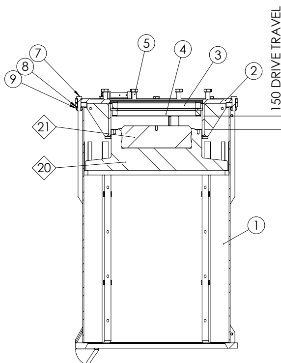
SECTION B-B SCALE 1 : 40
